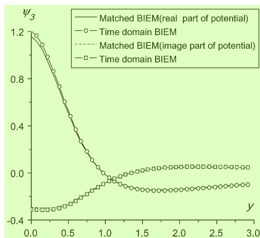
Fig. 3. The complex amplitude of potential on free-surface at Station 20. 9
