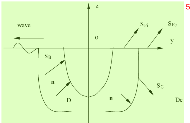
Fig. 1. Coordinate system and fluid boundary discretization. 6
