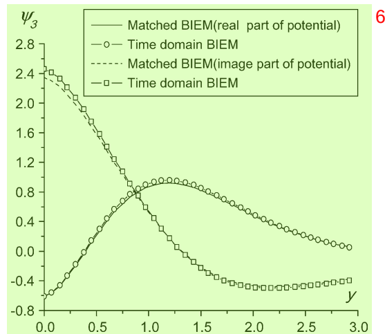
Fig. 5. The complex amplitude of potential on free-surface at Station 40.
