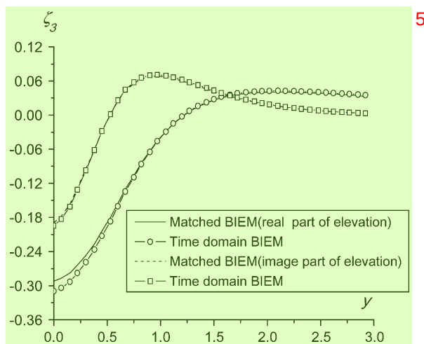
Fig. 7. The complex amplitude of wave elevation on free-surface at Station 20. 6
