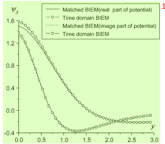
Fig. 4. The complex amplitude potential on free-surface at Station 30.
