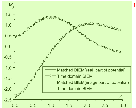
Fig. 6. The complex amplitude of potential on free-surface at Station 50. 2
